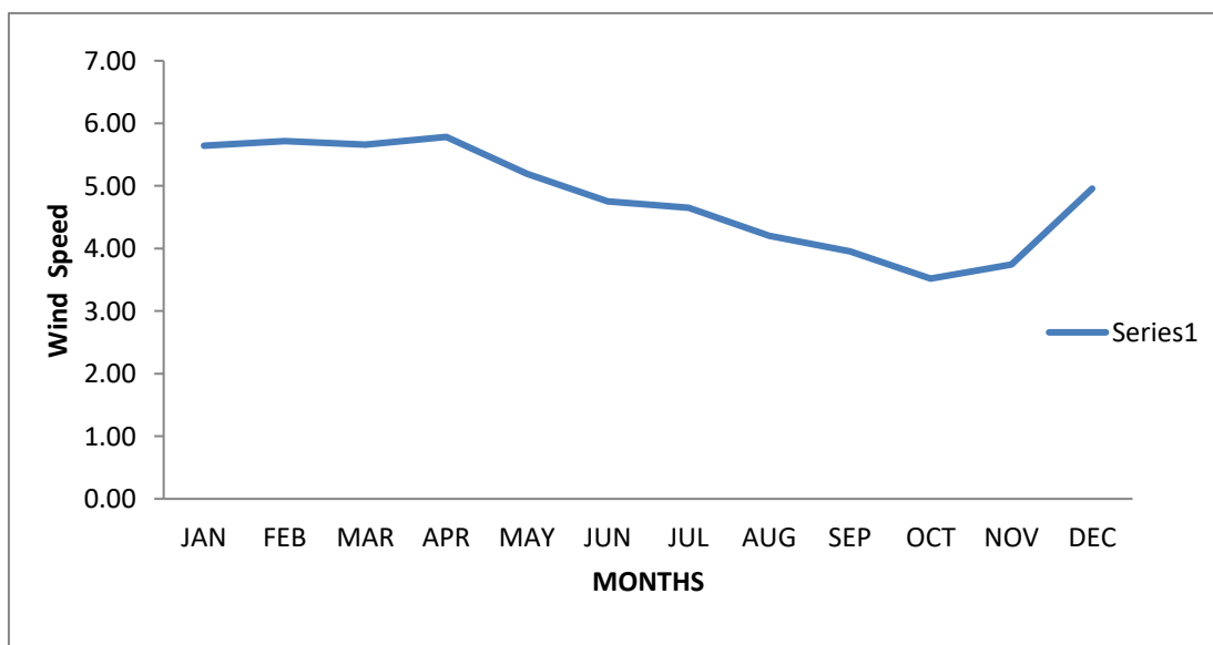
Figure 6: Monthly Wind Speed Variation over Fiidi, Makurdi (1986-2016)
