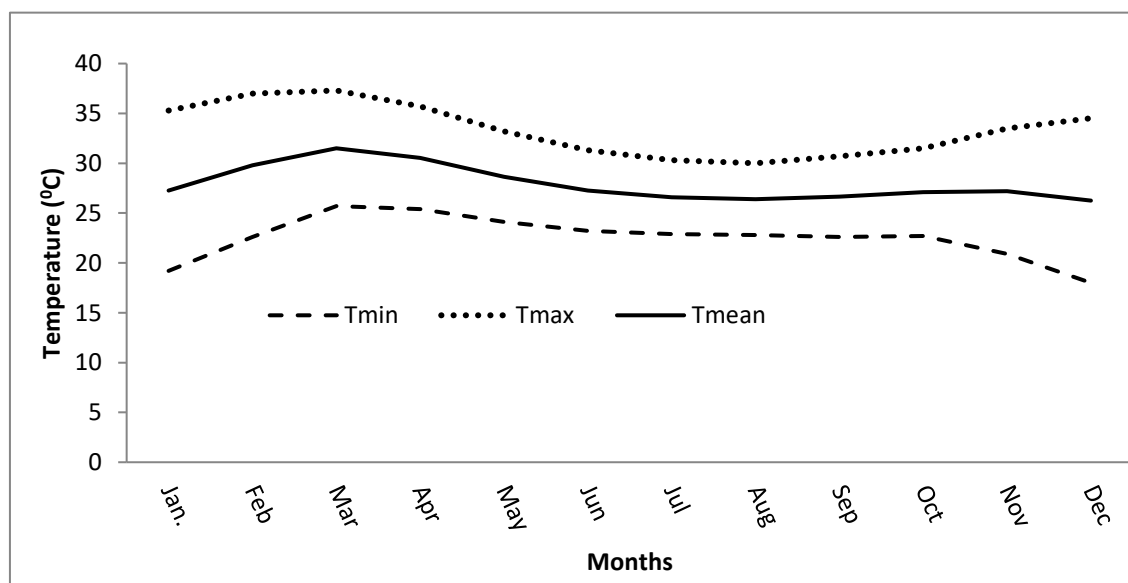
Figure 5: Monthly in Minimum, Maximum and Mean Temperatures over Fiidi, Makurdi (1986-2016)
