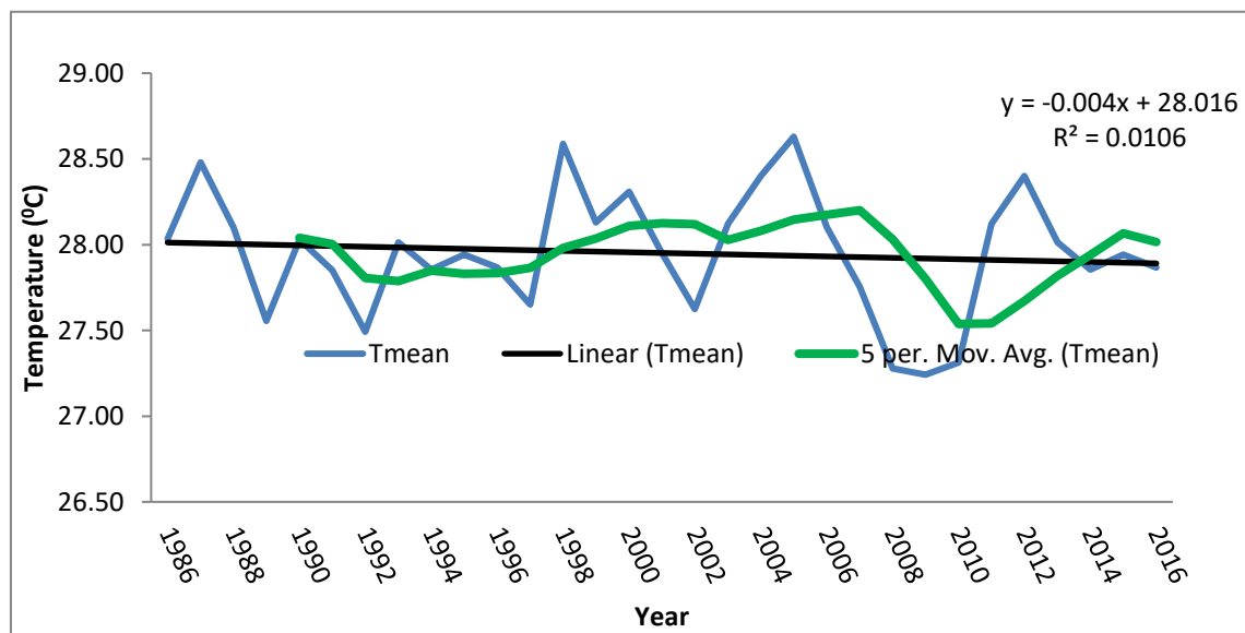
Figure 4: Annual Variation in Mean Temperature over Fiidi, Makurdi (1986-2016)
