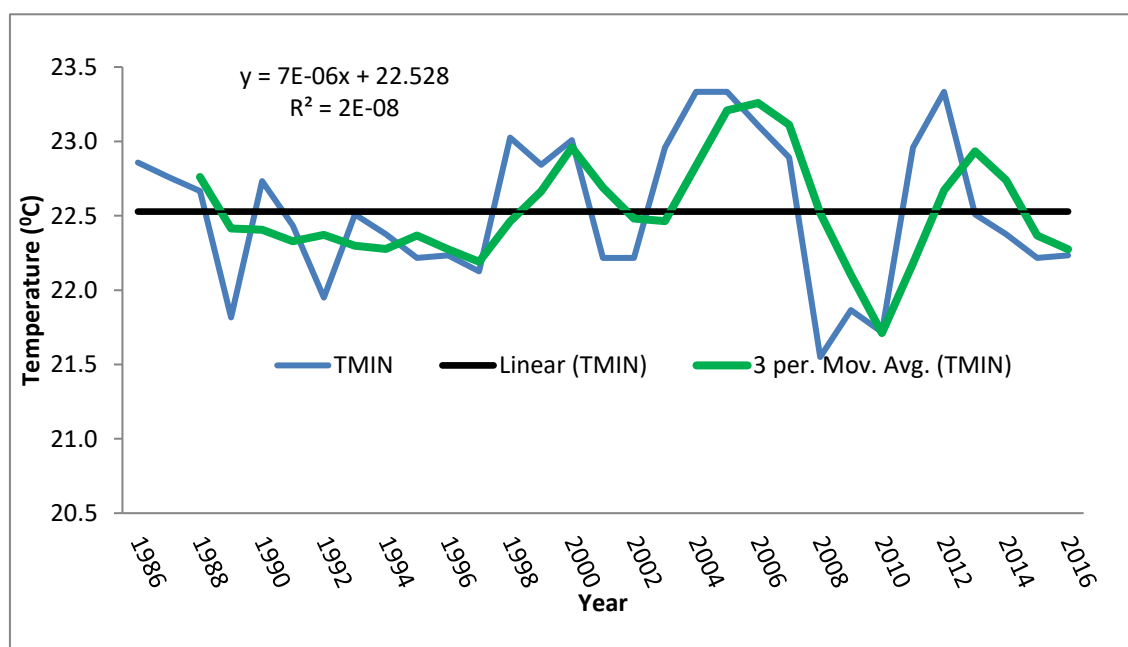
Figure 2: Annual Variation in Minimum Temperature over Fiidi, Makurdi (1986-2016)
