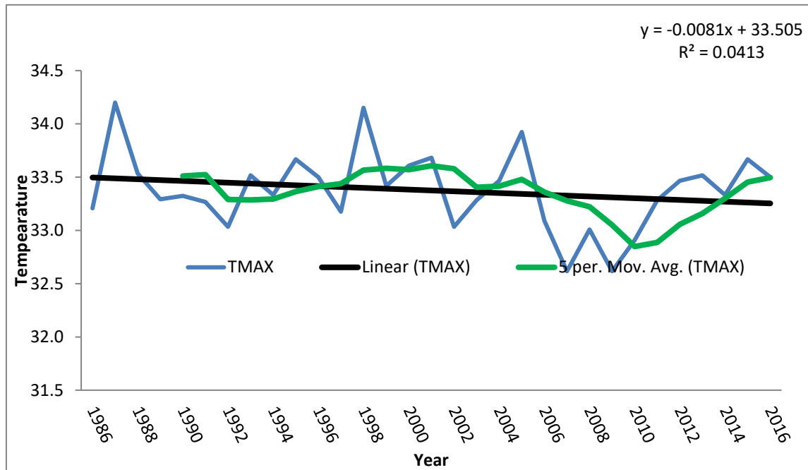
Figure 3: Annual Variation in Maximum Temperature over Fiidi, Makurdi (1986-2016)
