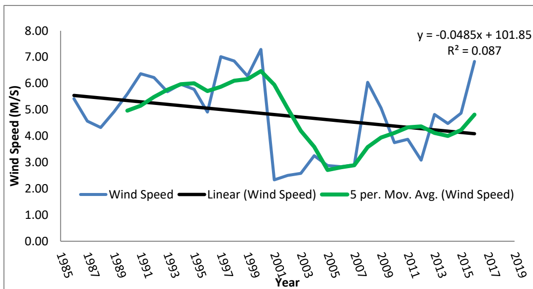
Figure 7: Annual Variation in Wind Speed over Fiidi, Makurdi (1986-2016)
