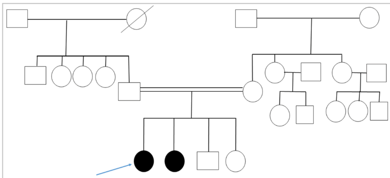
Figure 1 Pedigree chart
